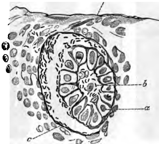
FIG. 90.—SECTION OF THE MUCOUS MEMBRANE OF A CHOLERA INTESTINE, X 600. A tubular gland ( a ) is divided transversely; in its interior ( b ) and between the epithelium and the basement membrane ( c ) are numerous comma-bacilli [after Koch].
